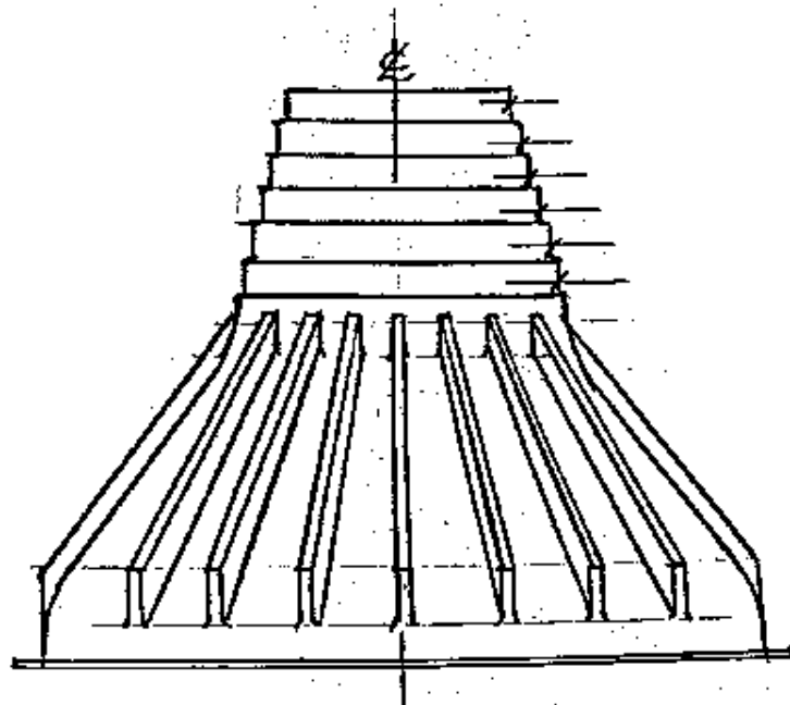
FIGURE 1—BIGFOOT SYSTEMS® FOOTING FORM
